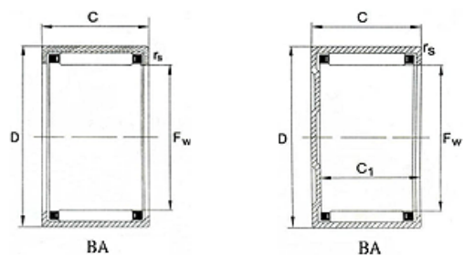
DRAWN CUP NEEDLE ROOLLER BEARINGS INCH SYSTEM BA
