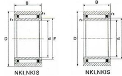
NEEDLE ROLLER BEARINGS WITH INNER RING: NKI,NKIS
