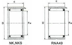
NEEDLE ROLLER BEARINGS WITHOUT INNER RING: NK,NKS
