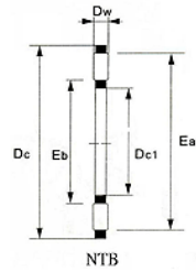
THRUST NEEDLE&RETAINER ASSEMBLY NTB
