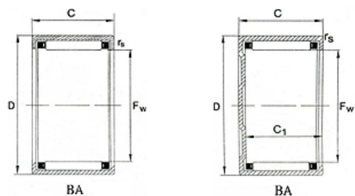
DRAWN CUP NEEDLE ROLLER BEARINGS INCH SYSTEM BA
